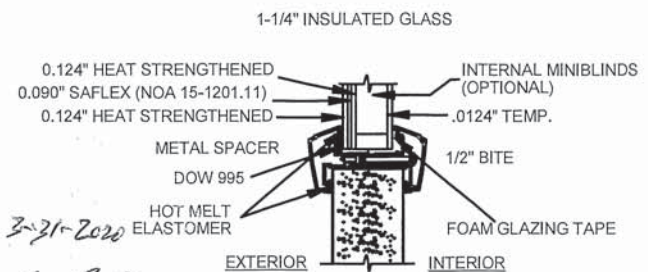
ALTERNATE GLAZING DETAIL IMPACT RATED GLASS
