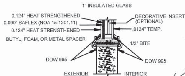
TYPICAL GLAZING DETAIL IMPACT RATED GLASS
